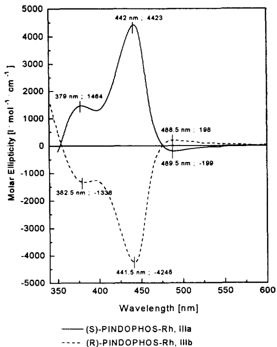
Figure 1. CD spectra of—(S)-PINDOPHOS-Rh, IIIa and --- (R)-PINDOPHOS-Rh, IIIb in methanol at 24°C
